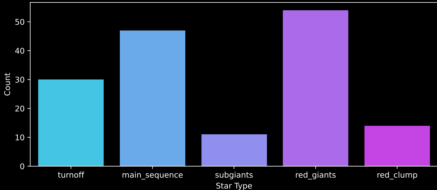
APOGEE DR17 Field: [K2_C4_172-20_btx] Count plot of Star Type
