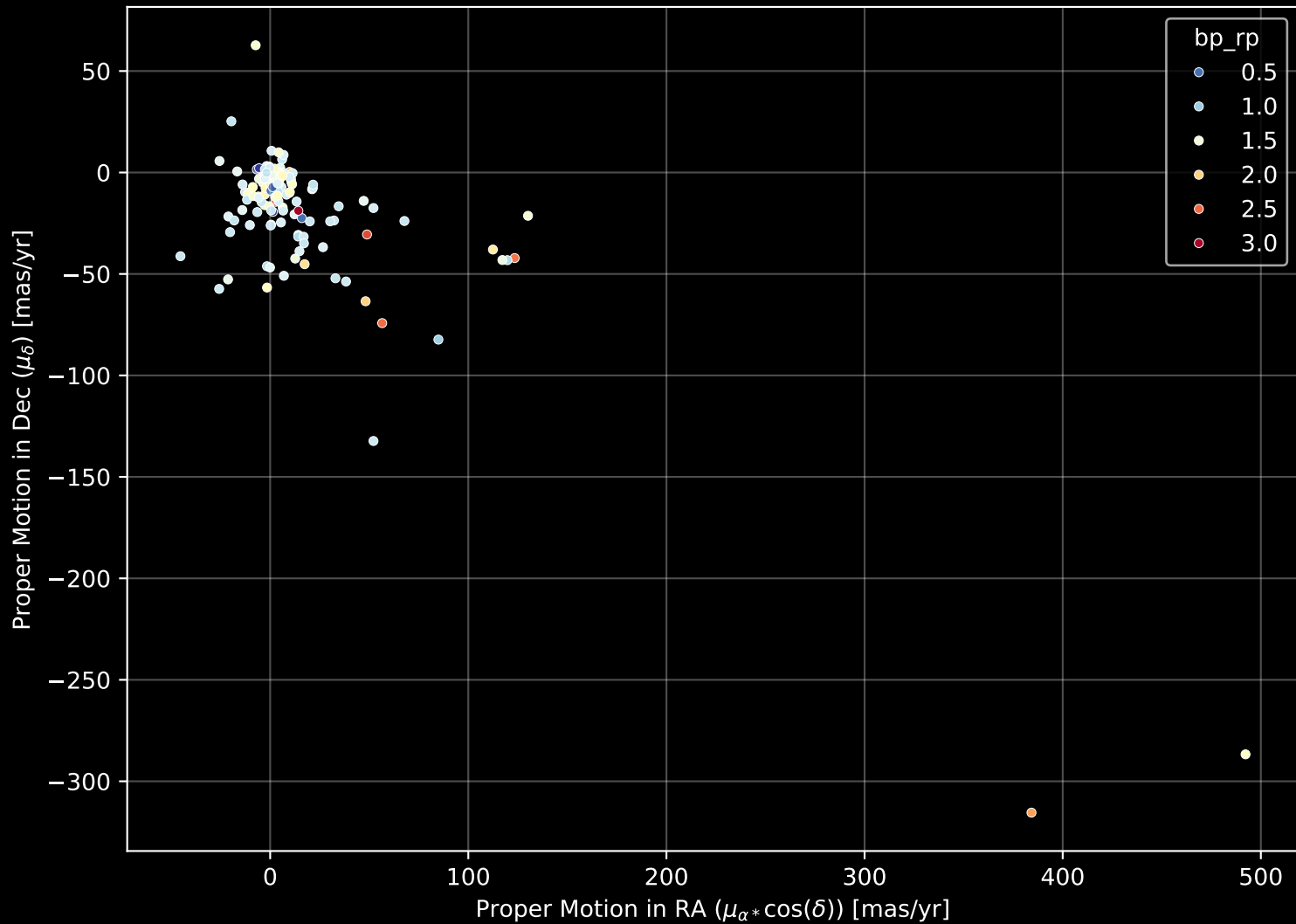
APOGEE DR17 Field: [K2_C4_172-20_btx] Proper Motion Diagram (n= 156)
