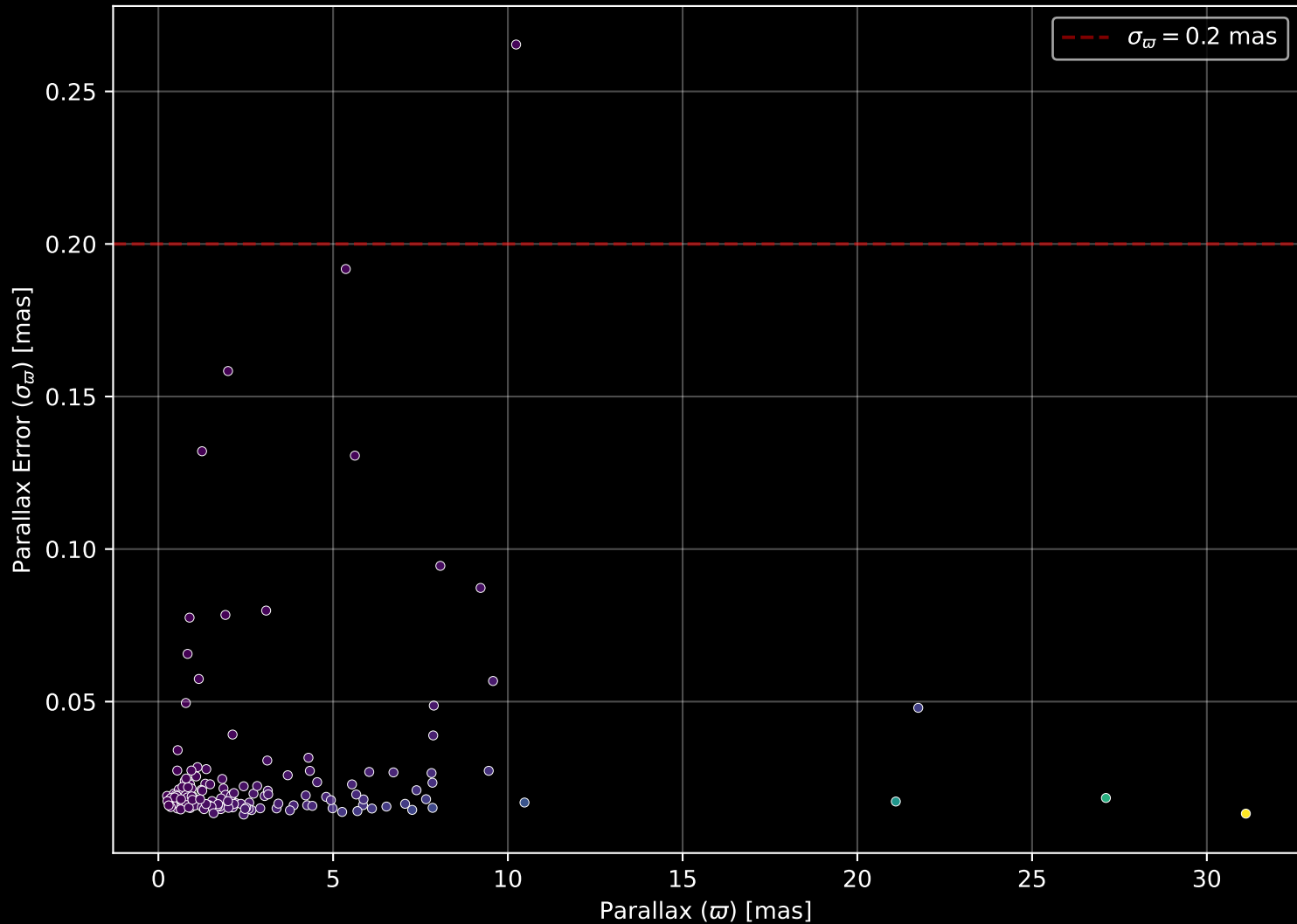
APOGEE DR17 Field: [K2_C4_172-20_btx] Parallax Quality (n= 156)
