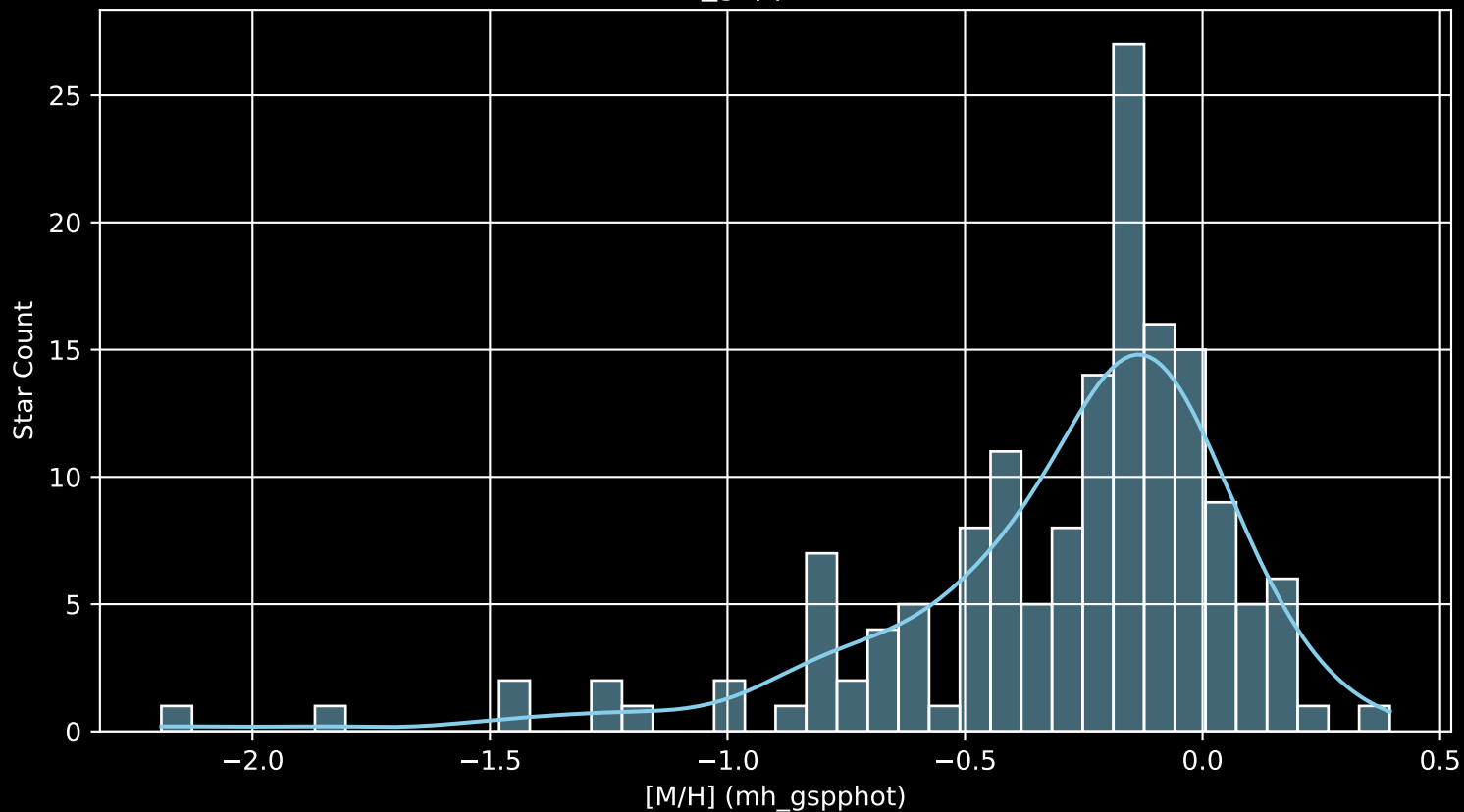
APOGEE DR17 Field: [K2_C4_172-20_btx [M/H] (mh_gspphot) (n= 155)
