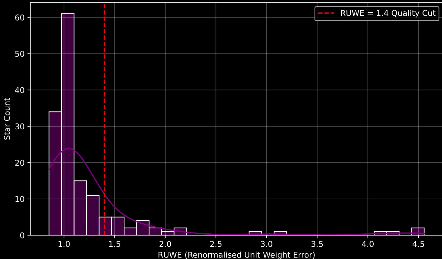
GAPOGEE DR17 Field [K2_C4_172-20_btx] RUWE Distribution (n= 148)
