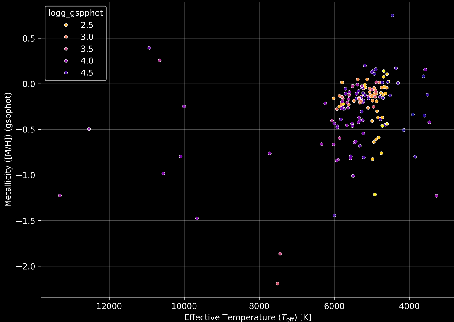
APOGEE DR17 Field: [K2_C4_172-20_btx] Stellar Population Parameters (n= 156)
