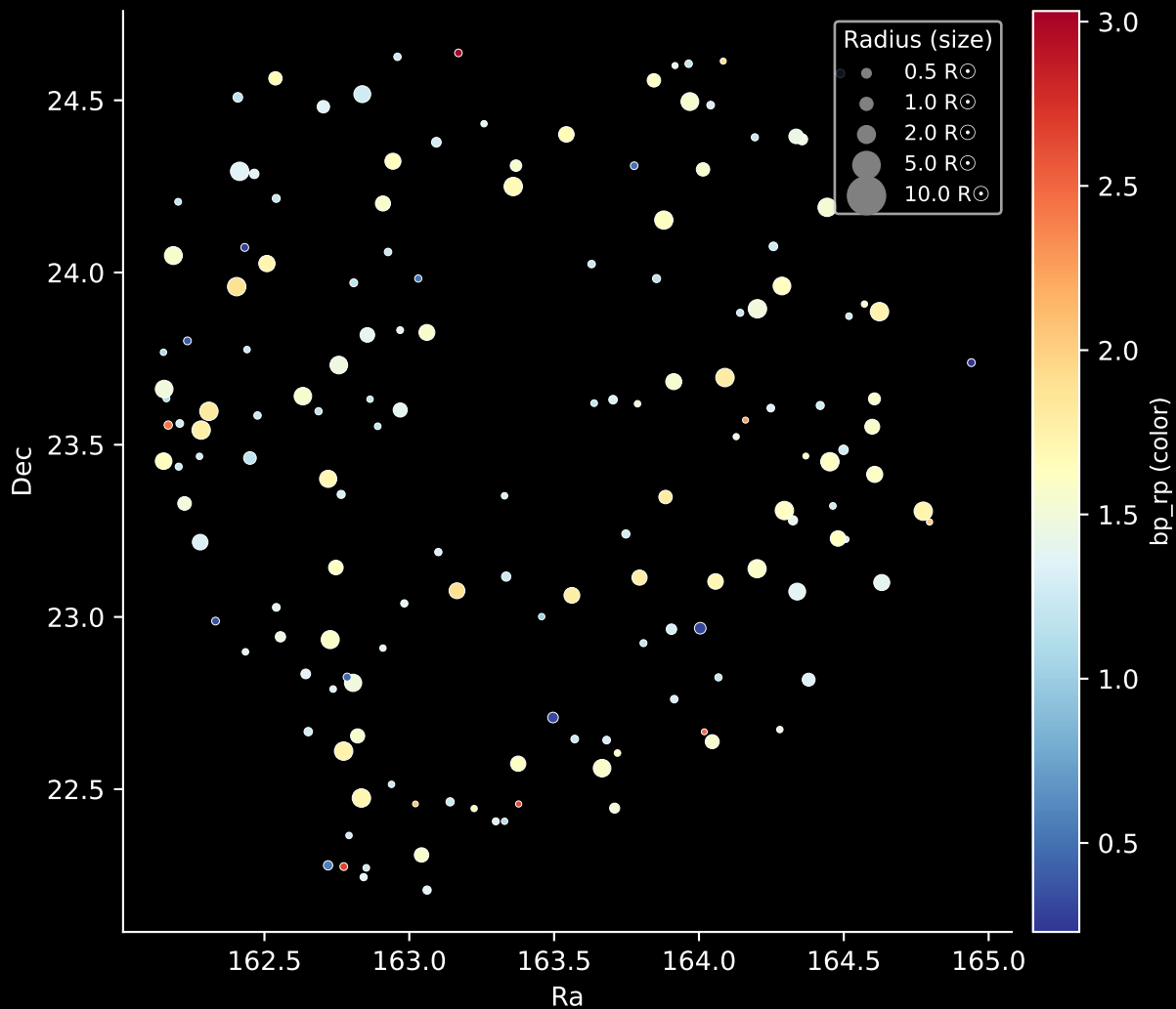
APOGEE DR17 Field: [K2_C4_172-20_btx] Stars: 156
